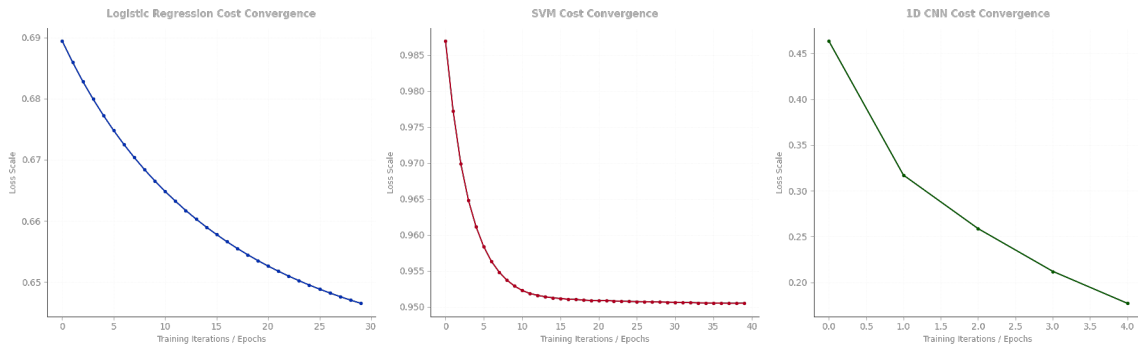
Logistic Regression Cost Convergence SVM Cost Convergence 1D CNN Cost Convergence
