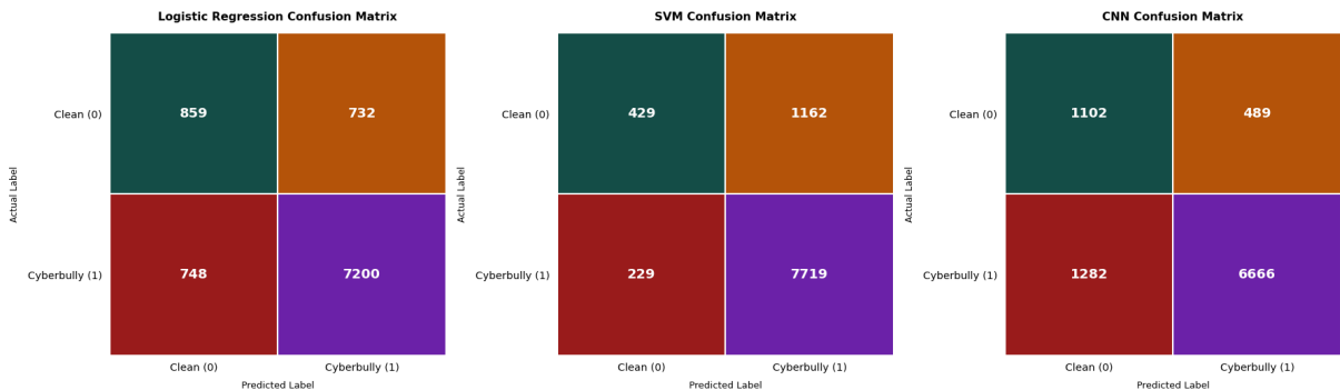
Logistic Regression Confusion Matrix SVM Confusion Matrix 1D CNN Confusion Matrix
